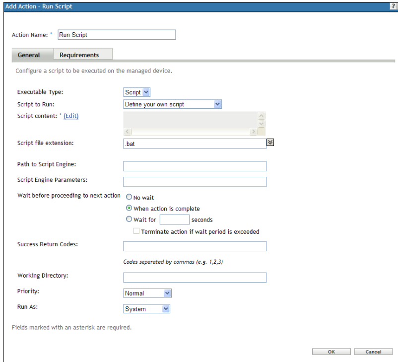
Figure 6-32 Action - Run Script Dialog Box with the Define Your Own Script option selected
